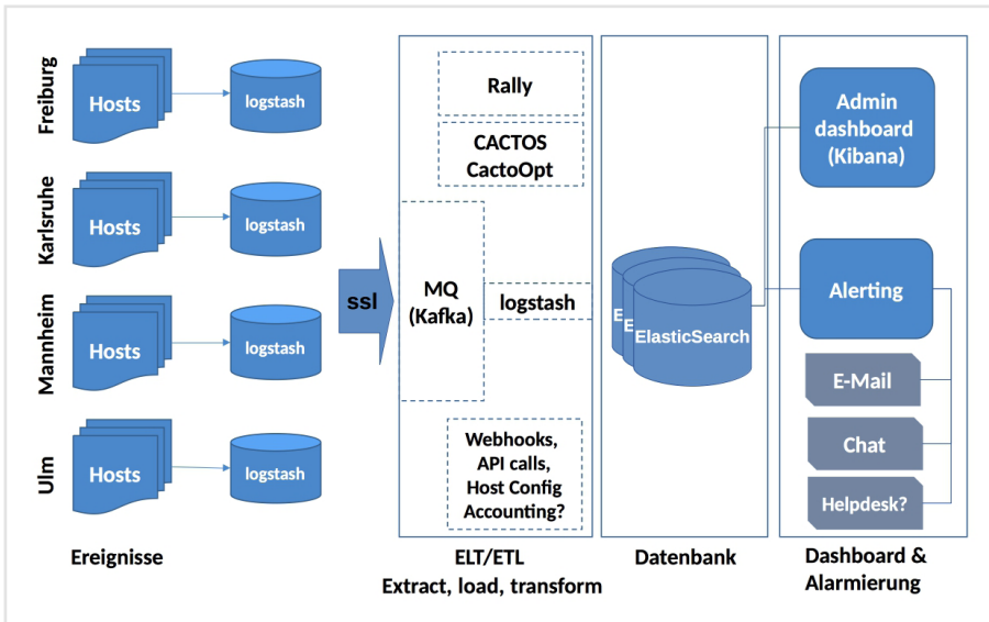
Abb. 4: bwCloud Eventprocessing
