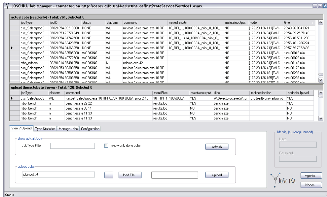
Abbildung 3: Jobmanagement-GUI
